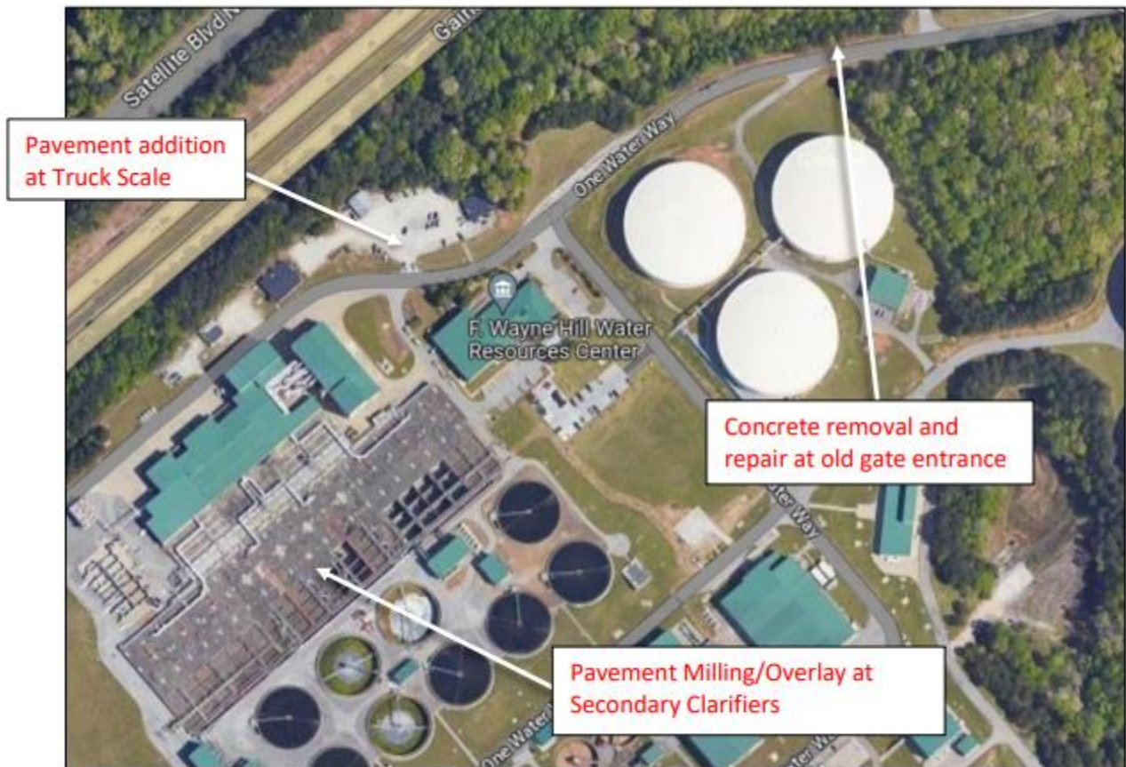
Figure 1 – Locations of pavement addition and rehabilitation areas at FWHWRC
