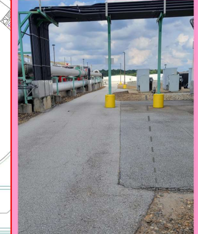
SAWCUT EXISTING PAVEMENT INTO THE DRIVEWAY BEYOND THE EXISTING JOINT.
