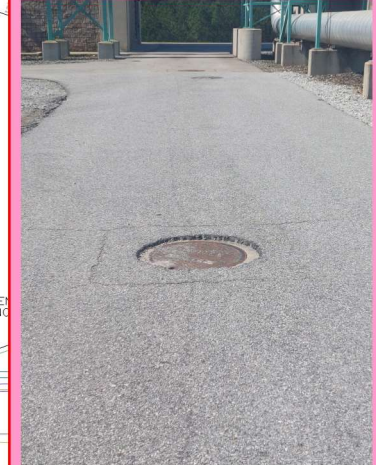
MILL DEPTH REQUIRED TO MATCH THE NEW PAVEMENT TO THE EXISTING MANHOLE AND CONCRETE COLLAR ELEVATION.
